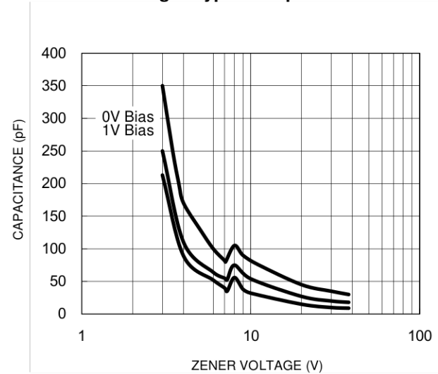
Fig.6 Typical Capacitance
