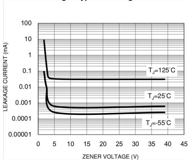
Fig.5 Typical Leakage Current
